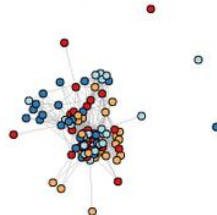
ChallengeRootOnly
